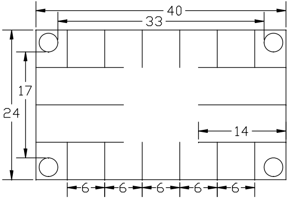
MOVING PLATEN LAYOUT
